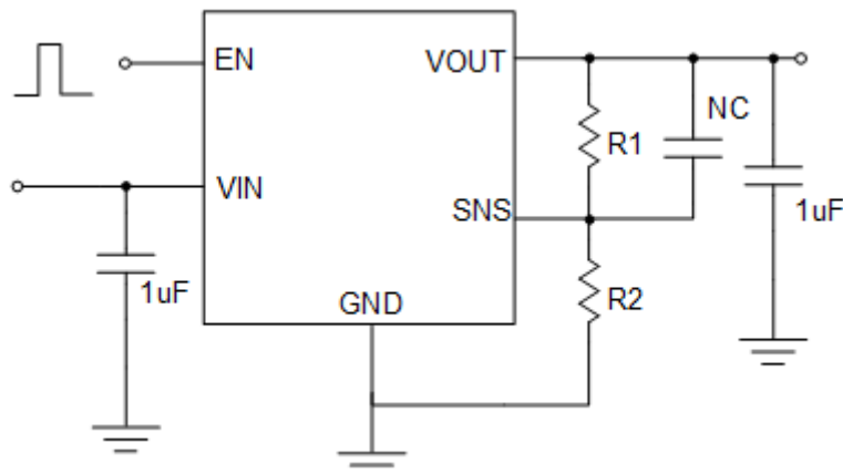
Figure 1 : Adjustable output voltage LDO application circuit
